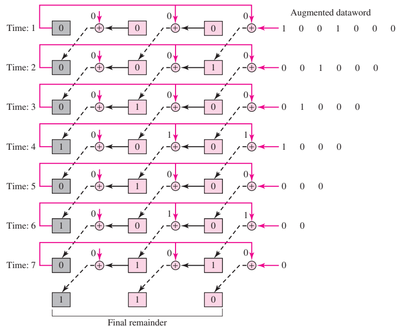
Figure 10.18 Simulation of division in CRC encoder
