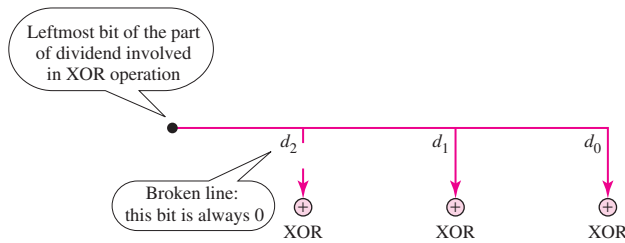
Figure 10.17 Hardwired design of the divisor in CRC
